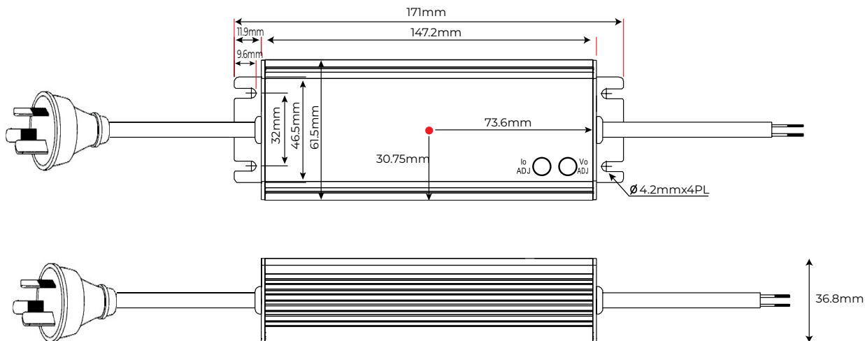
External Power Supply - Meanwell HLG-40H-15A IP65
