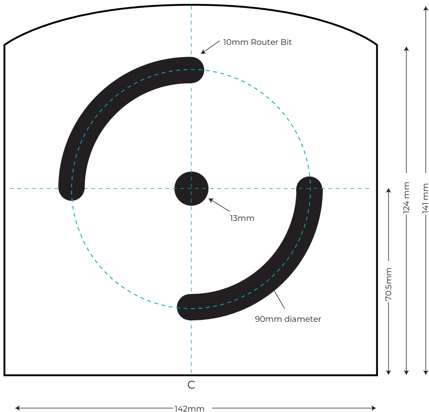
Base Plate
